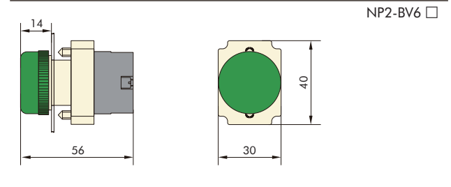
Dimensions(mm)
