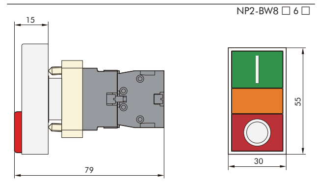
Dimensions(mm)
