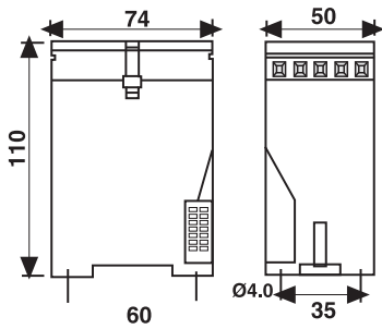
Size (Type PK 10)
