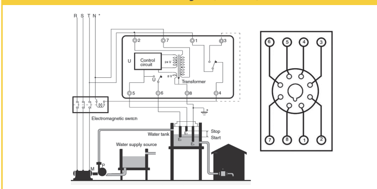
Connection Diagram (SSRC-04P)
