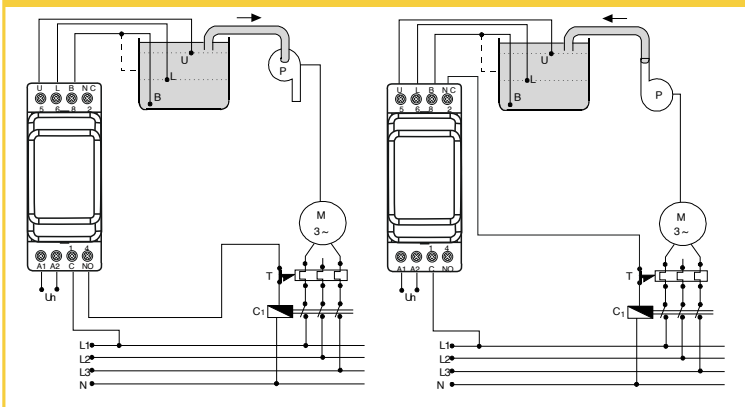
Connection Diagram (SSRC-04P)
