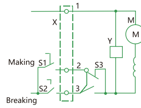
Without self-locking relay Specification AC 50Hz 230V or 400V
