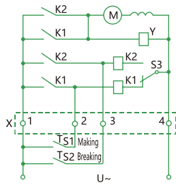
With self-locking relay Specification AC 50Hz 230V or 400V
