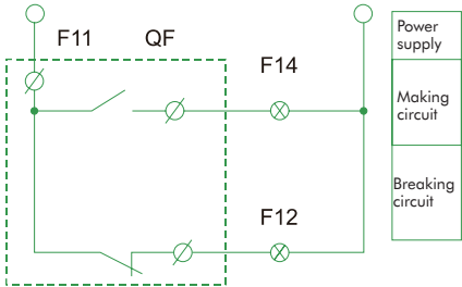
Wiring diagram of NM1 auxiliary contact
