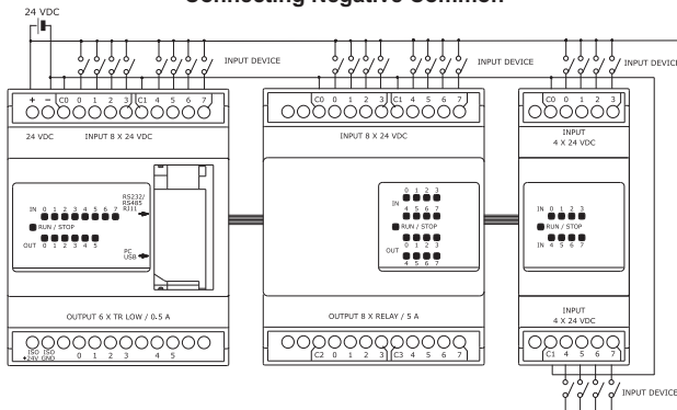
Connecting Negative Common
