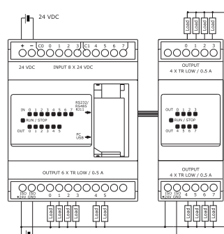
Connecting Low Side Output
