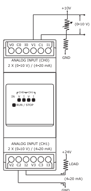
Connecting Analog Input Model
