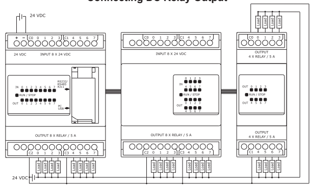
Connecting DC Relay Output
